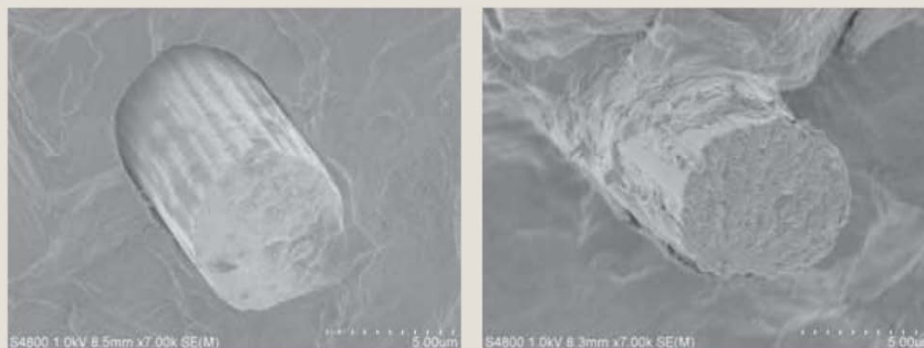
Photo 1 Interface between carbon fibers and PP resin (PP/carbon fibers = 70/30) Left: without UMEX, there are gaps at the interface due to poor adhesion Right: with 1% additives of UMEX, good adhesion is obtained
